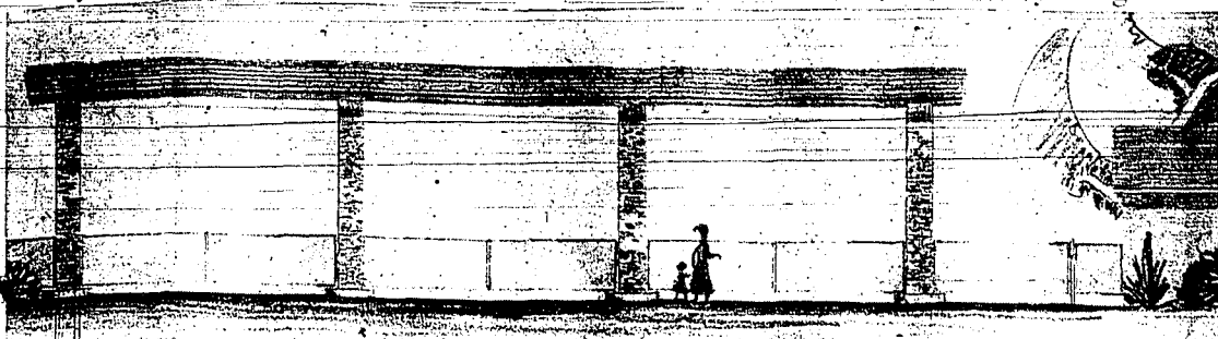
This drawing shows the proposed new entrance to the Twin Falls county fairgrounds in Flier, scheduled to be constructed during August. Drawn by Jack Christensen of Southern Idaho Drafting Service, the new entrance will be approximately 75 feet wide and will be built of Oatley rock or Mediterranean brick. Bids for the project are being received by the Twin Falls county commissioners and will be opened at 2 p.m. July 20.
