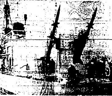
The USS Gyatt is shown at the Boston naval shipyard where she was commissioned as the navy's first guided missile destroyer. The Gyatt is equipped with Terrier guided missiles, shown above in launching position on stern of the ship. (NEA telephoto)
