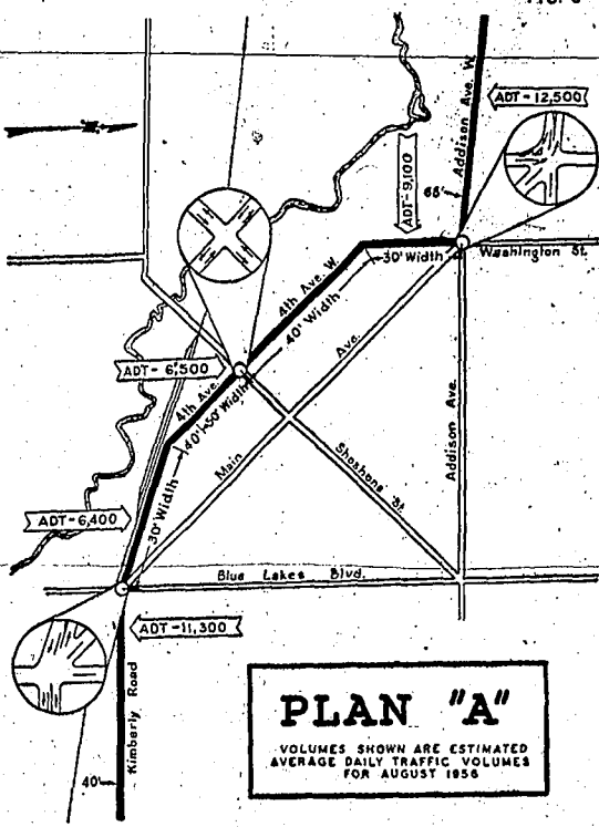
This diagram was prepared by the state highway department to show "plan A" for re-routing highway 30 through Twin Falls. The plan involves improvement of the present route or "truck lanes" from Five Points west to Five Points east. Diagram faces west. Average-daily traffic (ADT) figures are given for several points and insets show three intersections. (Staff courtesy.)
