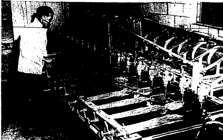
Steve Herrett, owner of the Herrett Gun-Stocks plant in Twin Falls, operates machine turning out 16 semi-finished rifle stocks at same time. Herrett, who is known throughout the gun world for his handgun stocks, only recently started turning out semi-finished rifle stocks. Last year, his plant here produced 8,000 stocks for handguns. (Staff photo-excraving)
