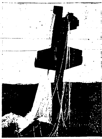
A Lockheed X-7 ramjet missile, its bright yellow point scorched black by air friction, is entangled in its own recovery parachute as it rests nose down at unditched proving ground. The missile, built by Lockheed at Sunnyvale, Calif., is used to prove powerful ramjet engines and has set a new speed mark making it the fastest air breathing vehicle in the U. S. (NCA telephoto)
