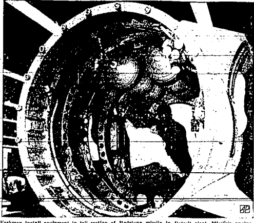
Workers install equipment in tail section of Redstone missile in Detroit plant. Missile's engine fits into this area in complete assembly. Modified Redstone was first stage of Jupiter C missile in launching U.S. satellite into orbit.
