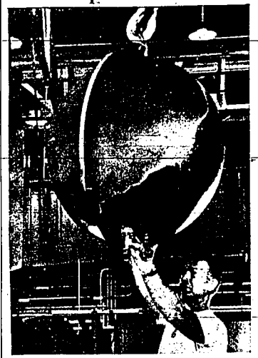
A North American Aviation workman in Los Angeles, Calif., checks this unique spherical hydrogen peroxide fuel tank, one of the many components being built into the X-15 research plane, which will fly at least 100 miles high, and at speeds greater than a mile a second. (NEA telephoto)
