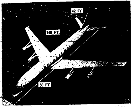
Painted an eye-catching red, white and blue, the first jet-ost model of the Douglas DC-8 jetliner is pictured outside its hangar at Long Beach, Calif. Scheduled for flight tests later this month and delivery to airlines in 1958, the DC-8 is powered by four turbojet engines. It will cruise at 500 miles per hour and carry between 110 and 116 passengers depending upon the seating arrangement. Staters domestic and foreign carriers have ordered 132 of the huge airliner which cost approximately five million dollars each. Among interior items are such things as reading lights, call bells, trash-air inlets, tables within reach of passengers and skyview windows. The DC-8 will be able to span the North America continent in less than five hours on regularly scheduled flights. (NEA telephoto)
