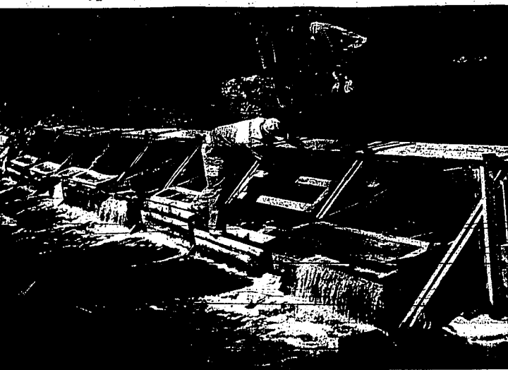
Inspecting the Wildhorse river weir, Keith Hawn raises the lid of one of the covered live boxes, while Robert Bell, project supervisor, looks on. The inclined-plane screens which strain the fish out of the water are on the upstream ends of the traps, on the approach to the live boxes. The Wildhorse river channel is beyond the trees. Downstream migrant salmon and steelhead follow diverted water from the Wildhorse river through a system of culverts to the weir where the ill-fated fish are strained out and retained in the live boxes until picked up for transport to their new habitat. (Idaho fish and game department photo-staff engraving)
