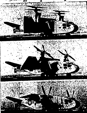
This sequence photo illustrates the wing-tilting action of Piper Aircraft's new X-18, "vertical take-off and landing" transport plane. The powerful twin turbo-prop-plus-jet engines can lift the plane straight into the air like a helicopter, then swing over forward and fly at high speed like any conventional plane. The X-18 was unveiled at Moffett field, Calif. For comparison of size, note man standing at left. (NEA telephoto)
