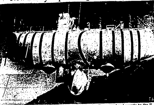
This is how the bathyscaph Trieste looks out of water. It was purchased recently by the U. S. navy from designer Augustus Piccard and is now being readied at the navy electronics laboratory.
