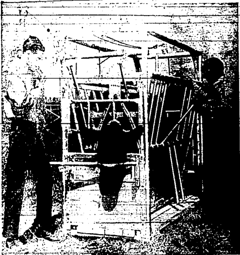
Greg Hollinger, left, and his father, Harvey Hollinger, Paul, demonstrate the branding and dehorning squeeze chute which won a national contest for the younger Hollinger, a senior at Minidoka high school. He received the $600 first prize in the welding contest. The chute was built at a fraction of what a chute would cost to buy. (Francisco photo—staff creating)
