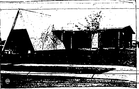
House with sandwich walls. This National Association of Home Builders research house in South Bend, Ind., has no frame, but is held up by pre-fabricated "sandwich" walls—wood outside and in with a layer of foamy plastic between.
