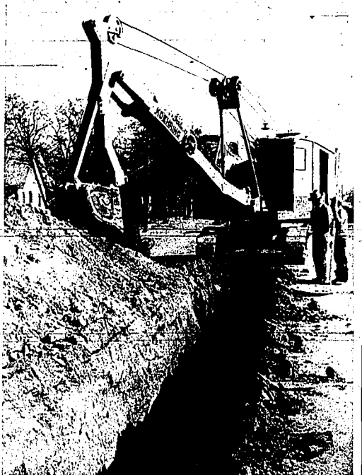
Workers began laying pipe Monday morning in the 500 block of Second avenue south for a storm drain which is part of the $700,000 Kimberly road project. A highway department spokesman said completion of the drain depends on arrival of the remainder of the pipe for the project. The overall project is slated for completion Oct. 1, 1960. (Staff photo-entouring)
