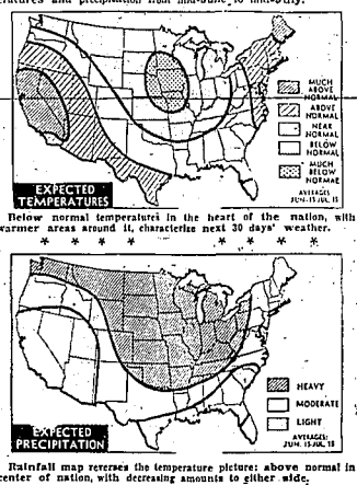
Rainfall map retunes the temperature picture: above normal in center of nation, with decreasing amounts to either side.
