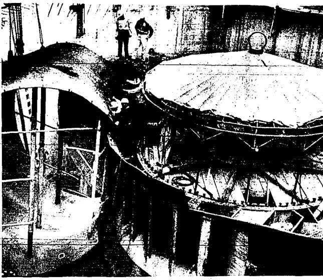
Construction of Oxbow dam has taken another step forward with installation of the first of the major scroll cases. The scroll case is being lowered into place in Oxbow's 200,000 kilowatt powerhouse.
