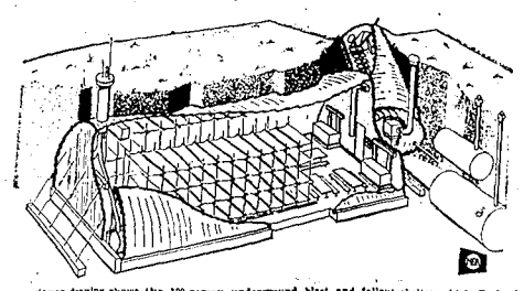
The cutaway drawing shows the 100-person underground blast and fallout shelter which Burbank, Calif., is proposing for its "neighborhood" approach to civil defense. The shelter was designed by the U. S. naval radiological defense laboratory at San Francisco. The model is at Camp Parks, Calif.
