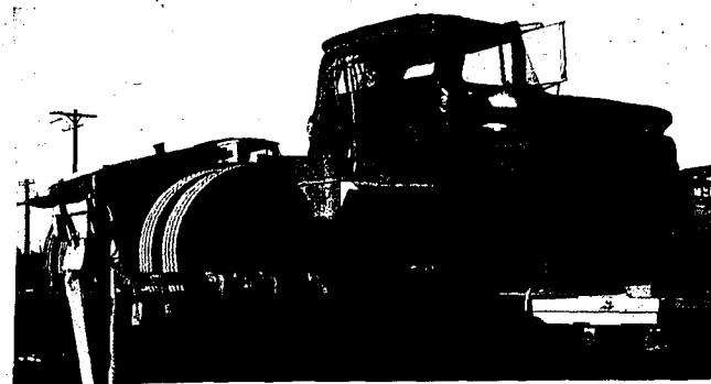
A specially equipped tractor cab backs onto a tractor off the recently installed Twin Falls loading ramp. The ramp enables the tractor to unload automobile carriers directly from a string of several flatcars and deliver configured goods directly to their destination.
