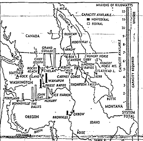
Development of further power resources in the Columbia river basin by joint U. S.-Canada action is proposed in a new treaty. Vertical lines at existing dams and those under construction show relative power potentials. Construction of three new dams in Canada—Arrow, Duncan and Mica—and at Libby, Mont., would add 1.6 million kilowatts of power to bring basin total to almost 20 million kilowatts. The U. S. cost would be 453 million dollars by 1970, 765 million by 1985.
