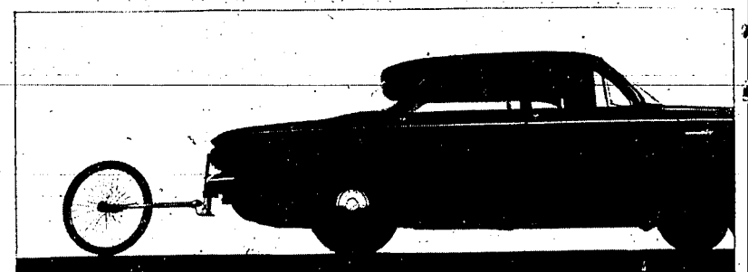
Shell test drivers add a "fifth wheel" to their cars for precise distance measurement during mileage tests. It helps them record performance to a decimal point.
