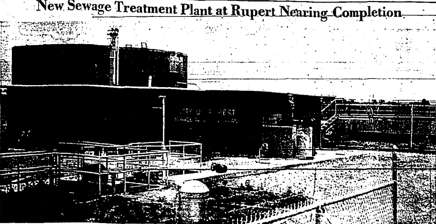
This new $385,000 sewage disposal plant constructed this summer just south of Rupert will be in operation soon, according to Rupert Mayor Gloyer Acock. The connecting lines and outfall lines to Snake River are all in readiness, with some electrical work and the installation of a motor remaining, he said. Reynolds Construction company, Twin Falls, is contractor for the project which is expected to handle the needs of the city for several years. (Staff photo-engraving)
