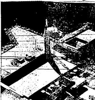
An Atlas intercontinental ballistic missile is ready for firing after having been raised from its horizontal underground launch box at operational base near Reading, Wash. Heavy doors slide open to expose the 65-foot missile. Ground opening at right is flame bucket door for release of exhaust. Trailer and test in foreground was for test and has since been removed. (AP wirephoto)
