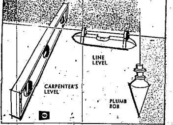
Don't count on your eyes when laying out vertical or horizontal lines in your work. These three levels are necessary for any home carpentry work.
