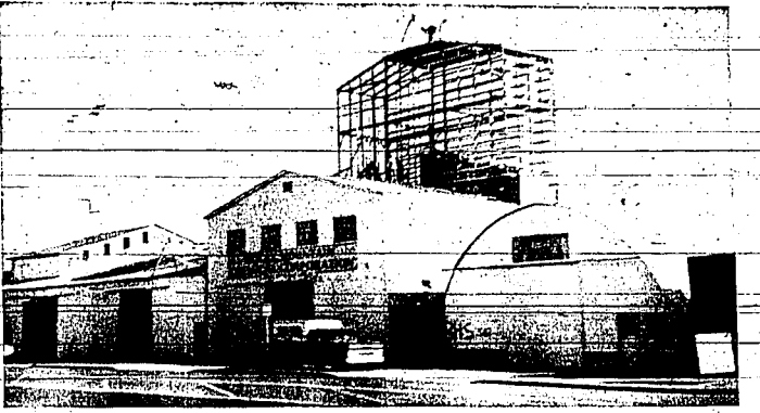
Elevator towers, part of the Rocky Mountain Chemical company's expansion program, are being rushed to completion with workers taking advantage of good weather. The company plans to expand its potato processing to include frozen French fries in addition to the commercial alcohol plant which was in operation last season. Company officials said the non-arrival of key machinery was holding up the installation of the French fry department, adding that some 50 per cent of the equipment is already here waiting to be put into place. The alcohol division of the plant is also undergoing extensive remodeling, they report. The total cost of the expansion program will run around a half million dollars, according to plant officials. They hope to be ready to begin processing before the first of the year. The plant will distribute frozen French fries and a frozen hot potato product under the Spring Hill brand. Besides the commercial alcohol, a mash used as a cattle feed is produced and sold. The company also plans to broaden its cattle feeding operations. This fall, officials report. (Staff photo- engraving)
