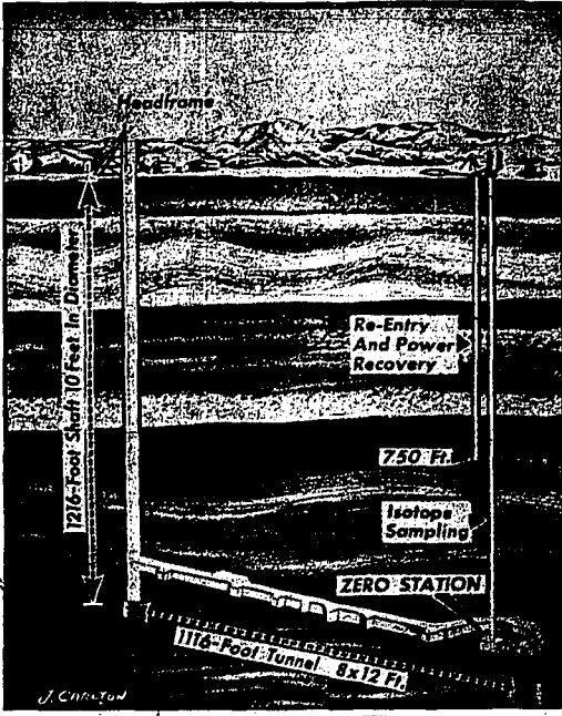
UNDERGROUND NUCLEAR TEST setup is shown in drawing prepared by atomic energy commission. Undergoing explosion is planned Sunday near Carlsbad, N.M. The ABC constituted the facility to house the blast for study of atomic energy for peaceful use. Zero station, lower right, is site of explosion. (AP wirephoto)
