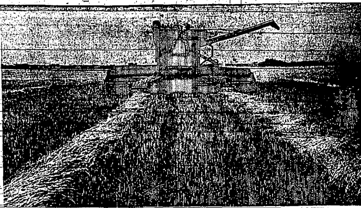
NEW DUAL PICKUPS permitting as much as 32 feet of wind-towed grain to be combined at a time will be available for John Deere 85 self-propelled combines for this year's harvesting. The new dual belt pickups will handle two windrows laid by a 14- or 16-foot windrower, and will permit combine owners to practically double the harvesting capacity of the big self-propelled units.
