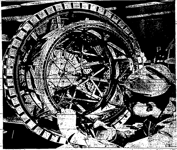
ELABORATE WIRING is required to interconnect the components of the Bell system's Telstar experimental communications satellite. Technician is preparing ends of cable wires. In background part of the frame work of another Telstar satellite being worked on can be seen. (American Telephone and Telegraph photo)
