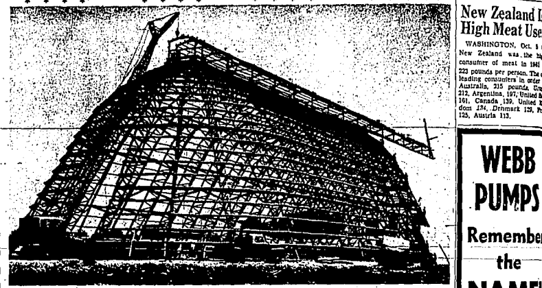
DURING CONSTRUCTION the new storage facilities building of the Amalgamated Sugar company in Twin Falls loomed large against the rural skyline. The steel girders, put in place by a huge crane, dwarfed the men crawling around on them. The warehouse, now completed and in use this week, is 380 feet long, 130 feet wide and 70 feet high. The storage portion will be unheated. It is covered with galvanized steel. (Times-News photo)
