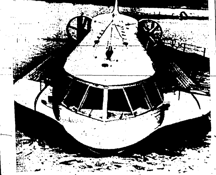
RUSSIA'S FASTEST RIVER ferry is this 50-passenger vessel, the Sarmovich, designed to ride nearly a foot above the surface of the water on a cushion of air. The Sarmovich, shown on a test run, is said to have a top speed of nearly 80 miles an hour. It can move over shallow water and can move into and out of the water on a sloping shore. The ship is about 28 feet long and 10 feet wide. The picture is from Soviet picture agency Tass. (AP wirephoto via cable from Moscow)
