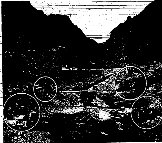
BIG HOLE for big dam. North America's deepest gorge will be even deeper when these four (count 'em) excavating machines complete a mammoth digging job now under way at Idaho Power Co.'s Hells Canyon Dam project. The machines, making rapid progress despite restricted work area in narrow canyon, are removing huge boulders and gravel from Snake River's former channel to reach solid rock on which new concrete dam will be built. Part of large construction force working around the clock, they'll excavate to a depth of about 100 feet. Drills will bore holes up to an additional 250 feet deep in bedrock for a pumped-in concrete mixture to prevent any seepage under the dam. Morrison-Knudsen Co., Inc., Boise, the general contractor, then will start building the 270-foot dam and powerhouse, scheduled for completion in 1968.
