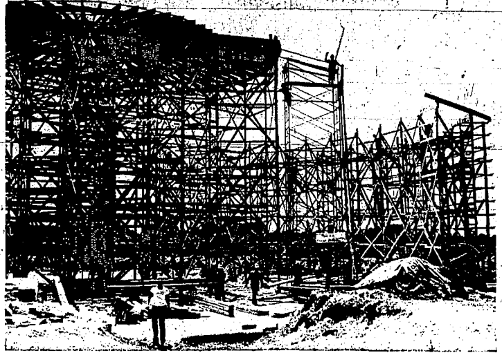
NEW FORMS FOR the five-million-gallon storage reservoir of the Twin Falls water development project are completed and workers for Crom Pre-stressing Inc. contractor have begun putting work on the first one-fifth of the reservoir structure. The complicated-looking maze of timbers
