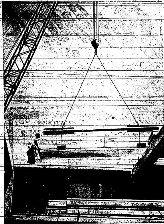
WORKMEN GUIDE A section of concrete flooring into place on the second story section of the new Twin Falls Clinic Hospital building under construction on Seventh Avenue North and Shoshone Street. The construction has drawn a number of spectators because of the methods being used to build the all-steel and concrete structure. Work is reported well on schedule with a completion date of Oct. 4 set by the hospital owners and Skyline Construction Co., Salt Lake City, Utah, contractor.
