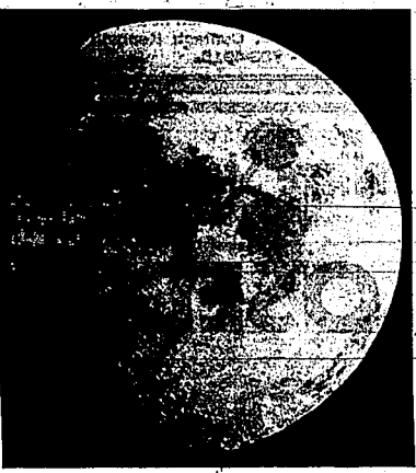
THIS PHOTOGRAPH of the moon was taken after the transfer injection, or breakout from lunar orbit to head homeward, when the Apollo 10 spacecraft was high above the lunar equator. The Apollo 10 landing site is near the lower left margin of the Sea of Tranquillity, which is the large dark area near the center of the picture. (UPI telephoto)
