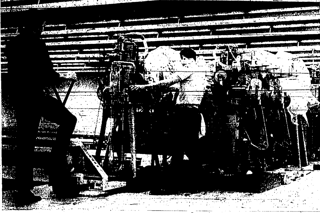
WORK ON THE NEW KELLWOOD CO. hosiery manufacturing plant on the south edge of Twin Falls continues, wet weather or dry, and here, inside the plant, it is dry. These workmen are seen moving special knitting machines into place inside the plant plant, Robert Matthews, plant manager, said 60 such machines are being moved into the building at the present time, and it is estimated about 500 of the machines will be in the building when operation gets under way. While work continues at the modern plant, training continues at the C. C. Anderson building in downtown Twin Falls. Mr. Matthews said recently it may be six weeks to two months before the plant is ready but an open house will be held this spring after the plant is finished and the machinery is in operation.
