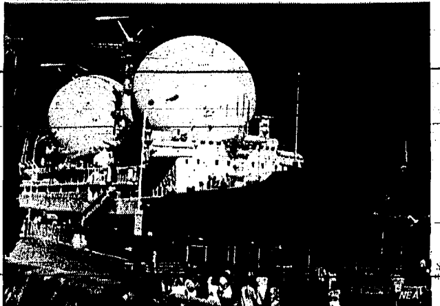
SPORTING TWIN RADAR DOMES, the world's largest space research vessel, the Soviet Union's Kozmonaut Vladimir Komarov, makes a striking study moored at the Yantla shipyard. The 18,000-ton ship can conduct observations not only of earth satellites, but also of automatic interplanetary probes, relaying data obtained to ground stations many miles away.
