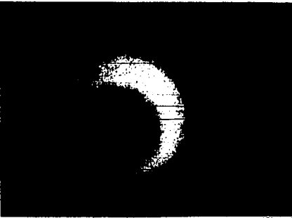
Photo gives clues to Uranus' atmospheric structure
