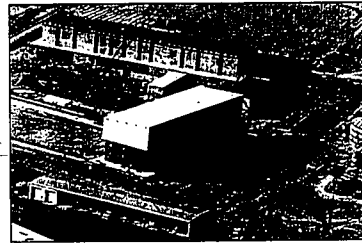
The white building at right weighs 120,000 tons and will ride on steel rails over buried waste in Pit 9 at the Idaho National Engineering and Environmental Laboratory. It will house remote retrieval equipment that will dig up waste to be treated in the gray concrete building.
