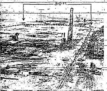
The job of providing housing for "monster airplanes like the U. S. S. Albatross" for the construction and engineer projects at the new dirigible base now being built at Subiway, Calif. Photo shows some of the work on the foundation for the big hangar. Dotted line shows the area to be covered, and figures indicate dimensions.
