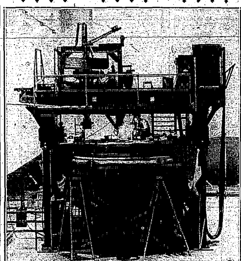
On this 50-ton machine progresses the work of grinding the 200-inch mirror, worth $2,000,000, for the huge telescope on Mt. Palomar, Calif., a scientific marvel that is expected to double the visible universe.
